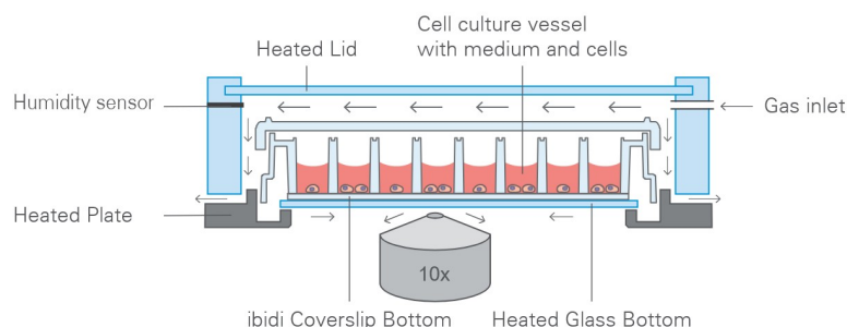
Figure 2.1: Diagram Showing the Airflow Path Within an Ibidi Multi-Well Incubator Chamber [1]
